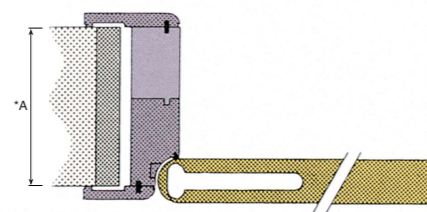
Stipite per muri a cm 18 - Door post for wall higher than 18
